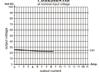
load diagram PSU25024-KS at nominal input voltage
